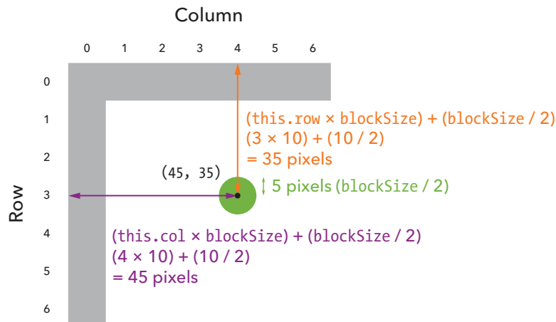
Figure 17-3: Calculating the values for drawing a circle
