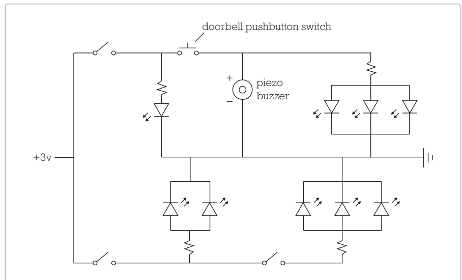
FIGURE 2-7: The full circuit diagram for the Switchbox
