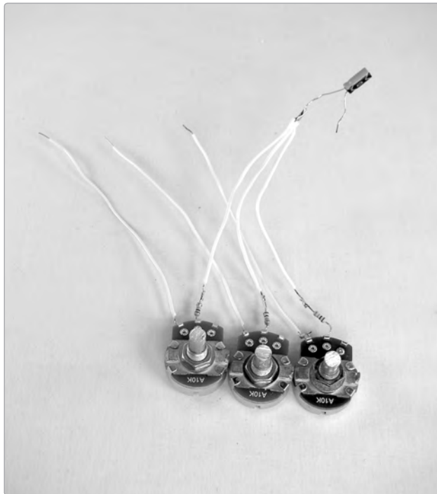
FIGURE 17-9: The three 10k pots wired up as a simple mixer; note that the shafts have been cut down
