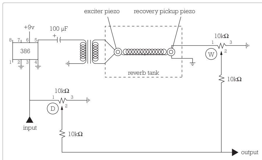
FIGURE 14-5: The schematic for the Spring Reverb
