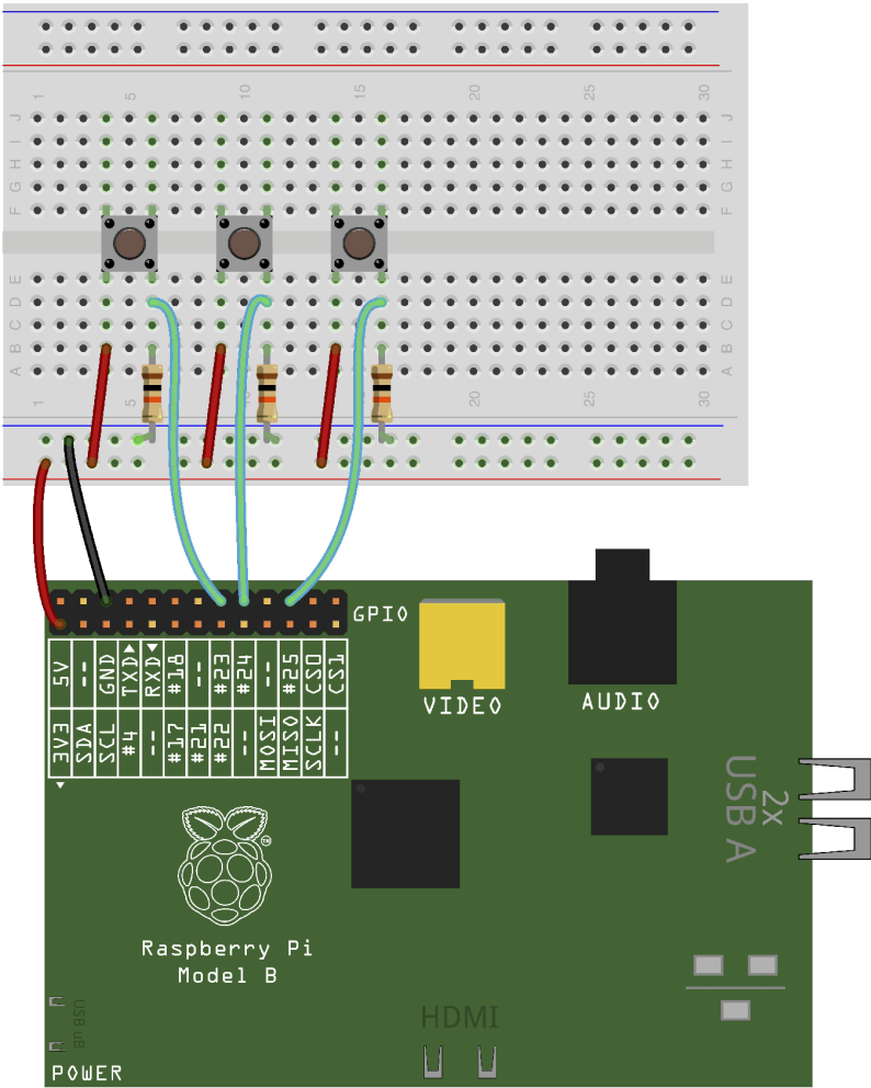
Figure 9-2. Completed circuit for the soundboard project
