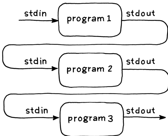
Figure 2-5. Pipes are a way of chaining smaller programs together to accomplish bigger tasks
