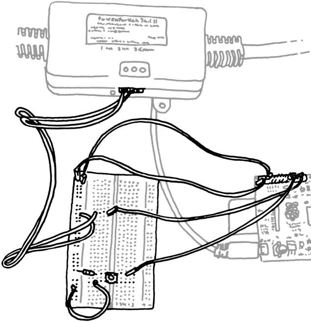
Figure 8-7. Connecting a PowerSwitch Tail II to the Raspberry Pi
