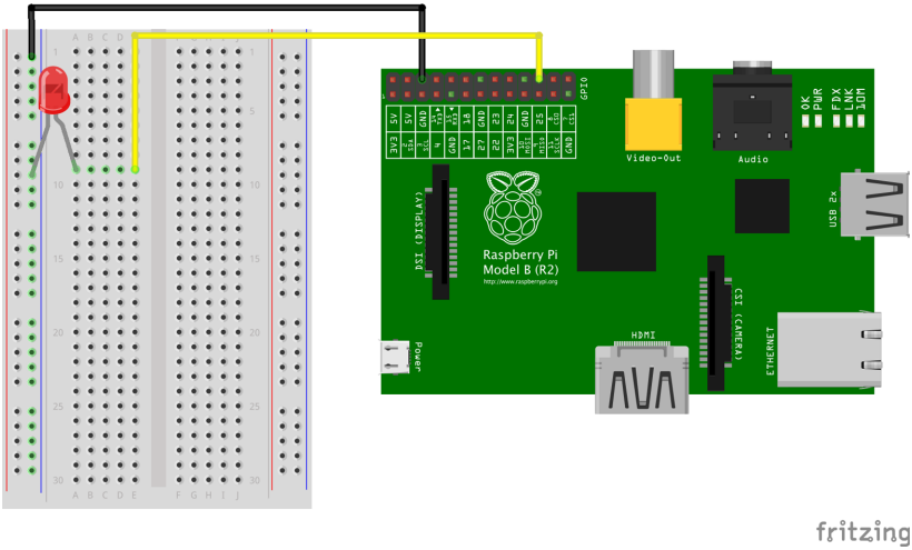
Figure 8-4. Connecting an LED to the Raspberry Pi
