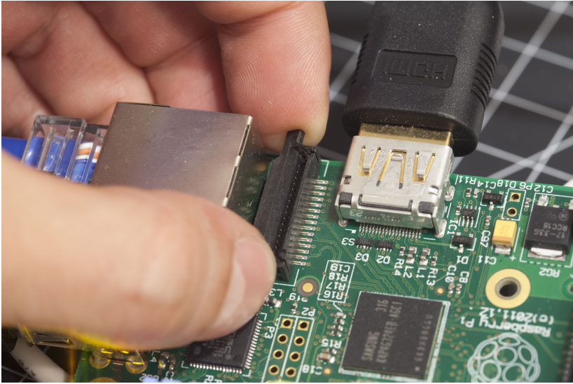
Figure 11-4. Opening the camera serial interface connector locking mechanism
