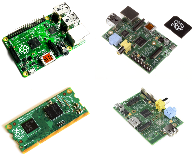
Figure 1-1. There are four versions of the Raspberry Pi: the Model B+, Model B, Model A, and Compute Module (clockwise from top). The Model B+ is the standard reference design. Model A photo courtesy of SparkFun Electronics (CC BY 2.0).
