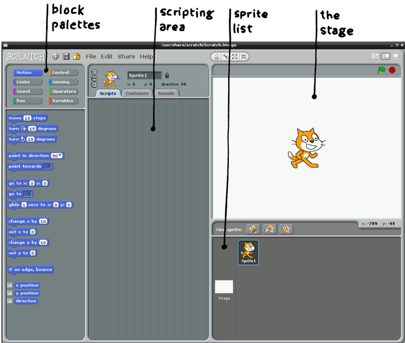
Figure 6-1. The Scratch environment; everything is contained in one window, with subpanels for the block palettes, the scripting and costume area, the sprite list, and the stage
