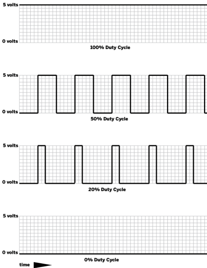
Figure 10-2. The duty cycle represents how much time the pin is turned on over the course of an on-off cycle
