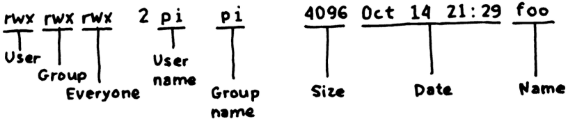
Figure 2-7. File permissions for owner, group, and everyone
