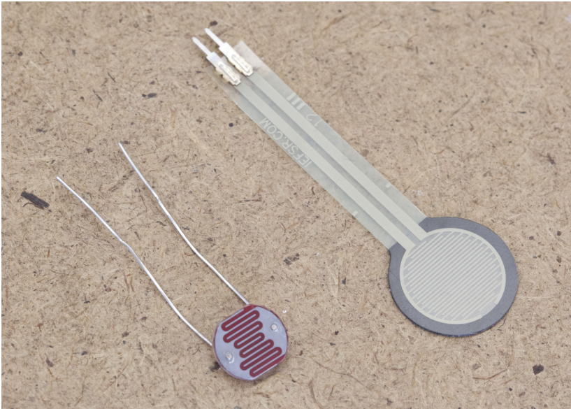
Figure 10-5. The photocell and force-sensitive resistors act as variable resistors and can be used as analog inputs
