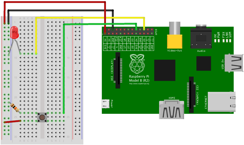
Figure 8-6. Connecting a button to the Raspberry Pi
