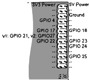
Figure 8-2. The default GPIO pins on the Raspberry Pi. In recent revisions of the board, GPIO pin 21 was swapped for GPIO pin 27. The Model B+ has additional pins below these, but the pin assignments for the first 26 pins are the same as the Model B v2.
