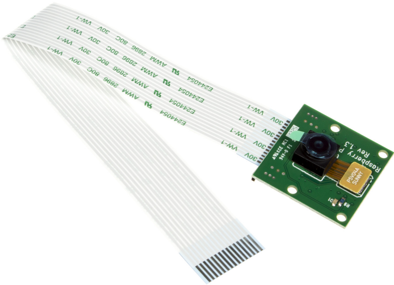
Figure 1-4. The 5 Megapixel Raspberry Pi camera module connects directly to the CSI connector. Although the camera module is very affordable at $25, the lack of focusing optics (and sensitivity to static) may or may not be the best fit for your project. See Chapter 11 for a full discussion of camera and the Pi.
