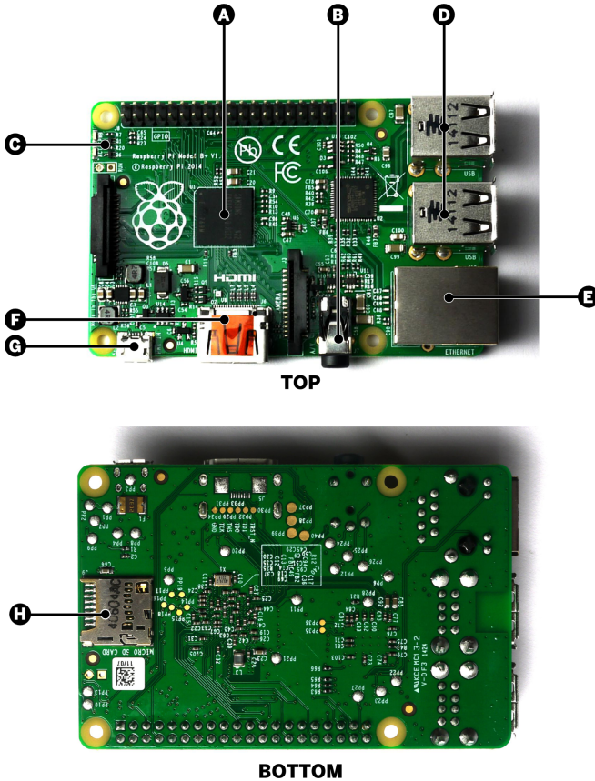
Figure 1-2. A map of the hardware interface of the Raspberry Pi
