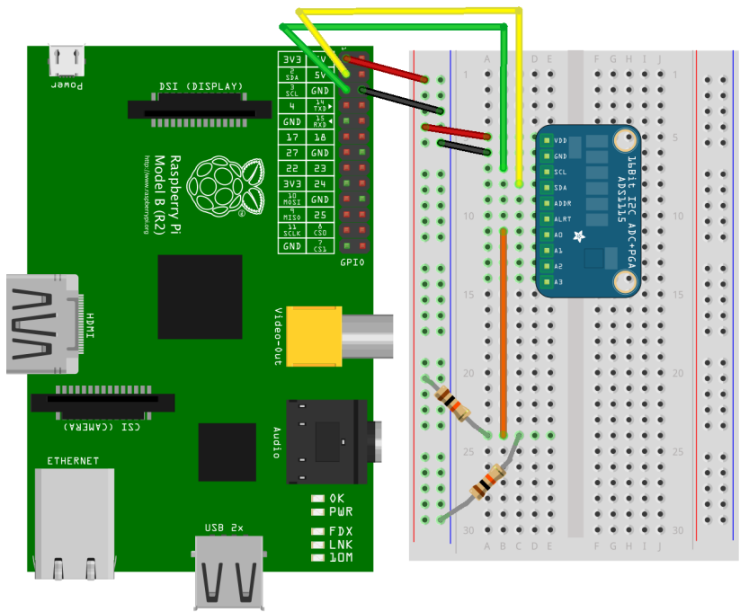
Figure 10-6. With two of the same value resistors between voltage and ground, the voltage between the two would be half of the total voltage
