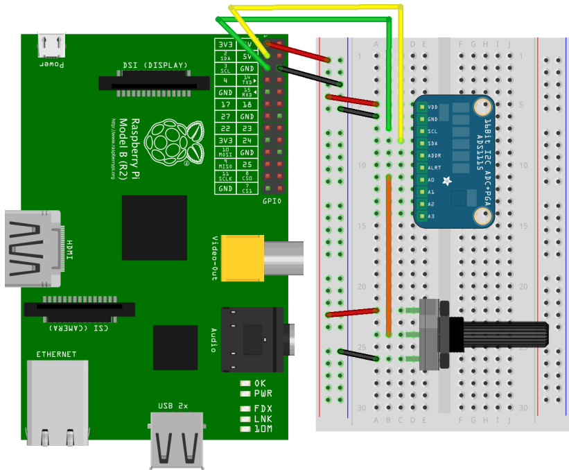
Figure 10-4. Using the ADS1115 to connect a potentiometer to the Raspberry Pi
