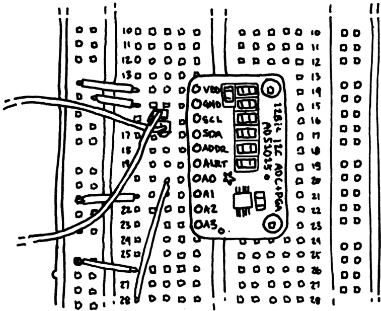
Figure 10-3. The ADS1115 analog-to-digital converter breakout from Adafruit
