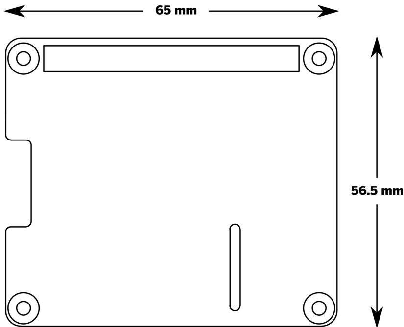
Figure 1-6. A Raspberry Pi HAT is an add-on board that conforms to a certain size ( 65 \times 56 \text{ mm} ) and has an EEPROM on board to help the Pi autodeTECT the functionality of the board, among other requirements. The full spec is available on the Raspberry Pi Foundations's GitHub page .
