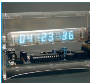
Ice Tube Clock Kit MKAD16 / $85.00
