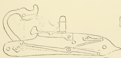
Matchlock of musket temp. William III.
