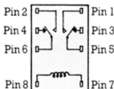
Circuit diagram for double-pole relay
