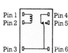
Circuit diagram for single-pole relay
