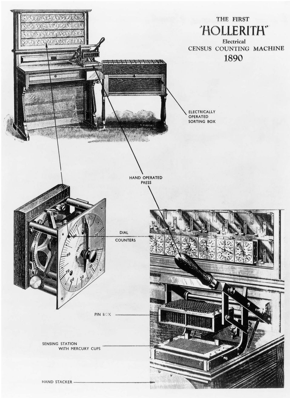
Hollerith Census Counting Machine: Hollerith's Census Counting Machine cut the time for computing the 1890 census by an order of magnitude. (Courtesy of IBM Archives)
