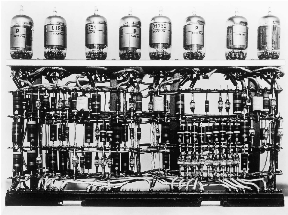
Vacuum tubes: In the 1950s computers were filled with vacuum tubes, such as these from the IBM 701. (Courtesy of IBM Archives)
