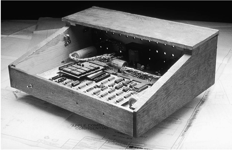
The Apple I: Steve Wozniak's original Apple I was a circuit board. (Courtesy of Apple Computer Inc.)
