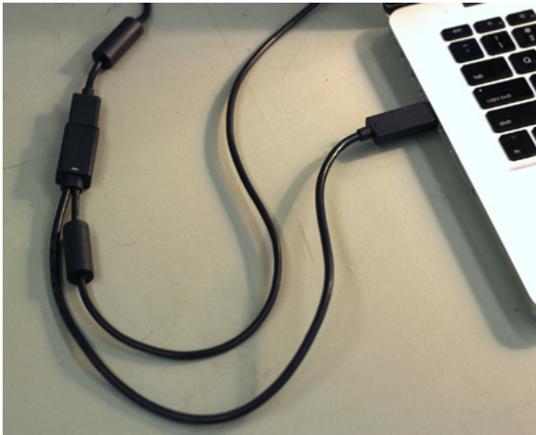
Figure 2-6. The male USB connector from the power supply plugs into your computer's USB port. With the Kinect plugged into the Xbox plug and the power plug in a socket, this completes the physical setup for the Kinect.
