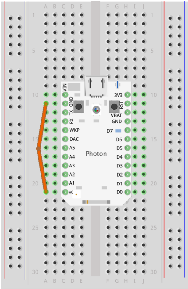
Figure 5-14. Connecting A0 to GND
