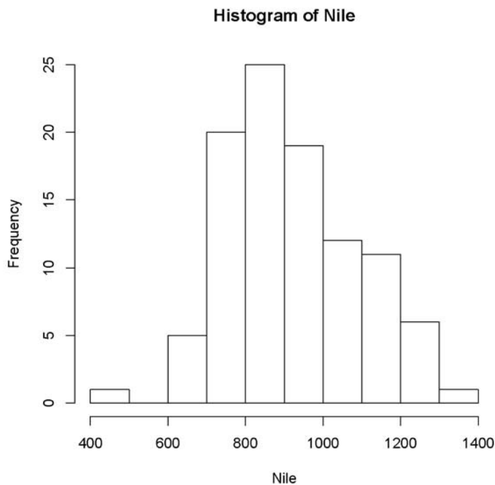
Figure 1-1: Nile data, plain presentation
