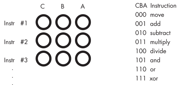
Figure 9-2: Encoding instructions
