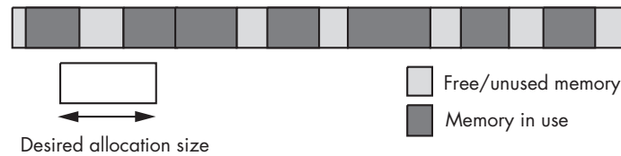
Figure 11-8: Memory fragmentation
