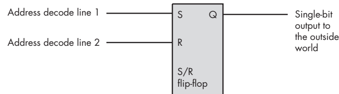
Figure 12-4: Outputting data to a port by simply accessing that port
