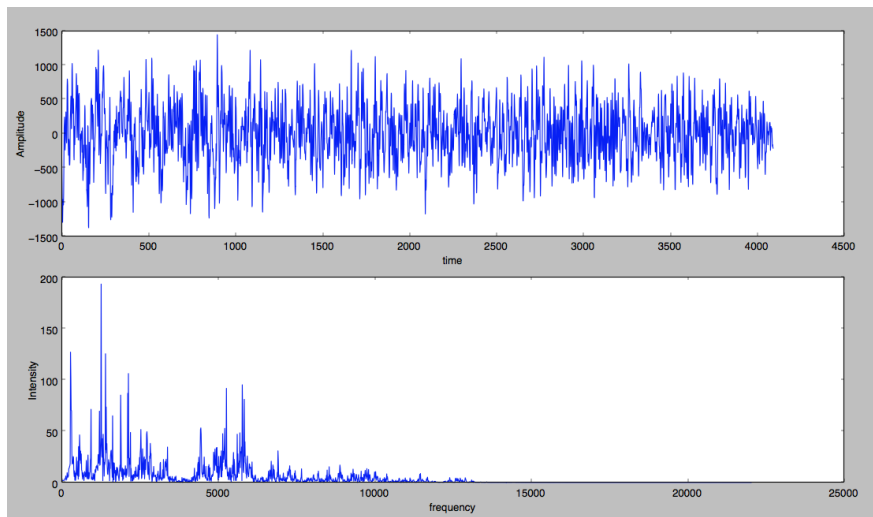
Figure 13-5: The FFT algorithm takes an amplitude signal (top) and computes its component frequencies (bottom).
