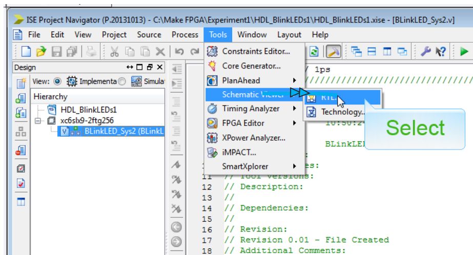
Figure 2-32 Launch the RTL schematic viewer
