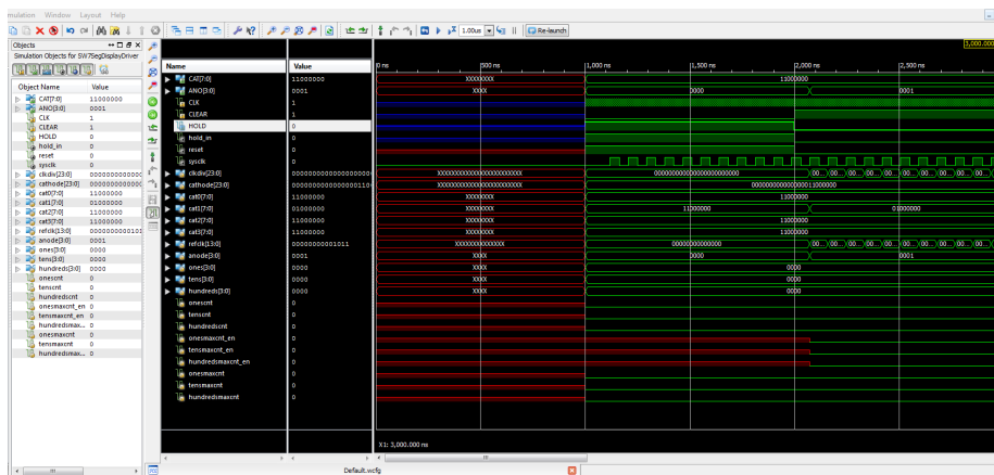
Figure 3-11 DOA simulation
