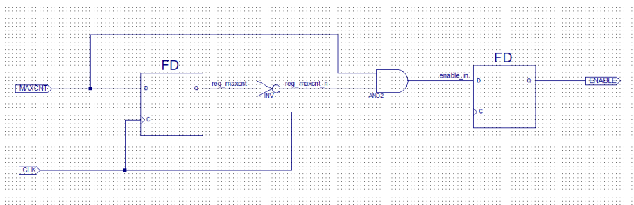
Figure 3-8 Schematic
