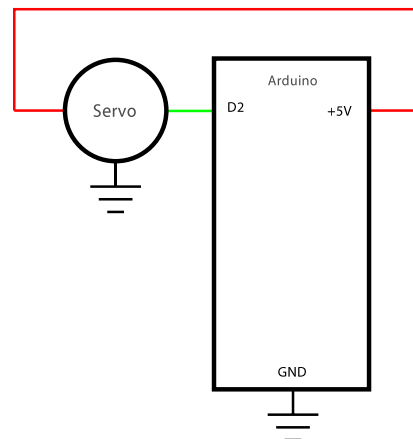
Figure 8-6. Connection diagram
