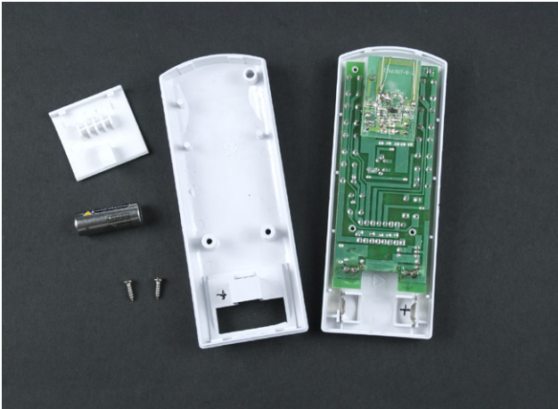
Figure 7-10. Opened remote control
