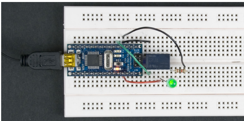
Figure 7-5. Connecting the LED with a relay
