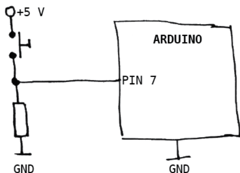
Figure D-5. A pushbutton connected to an Arduino digital input
