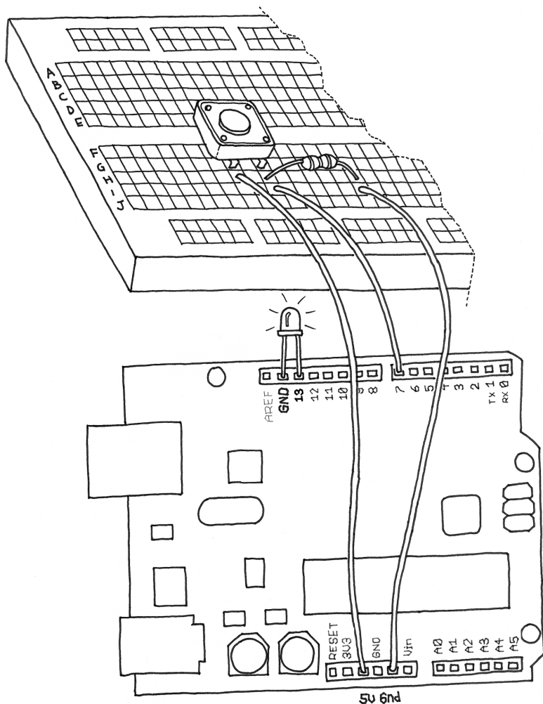
Figure 4-5. Hooking up a pushbutton
