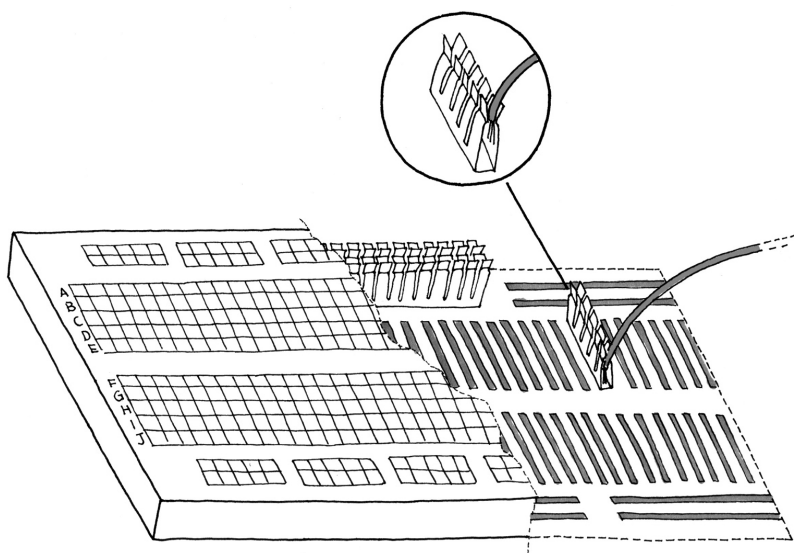
Figure A-1. The solderless breadboard
