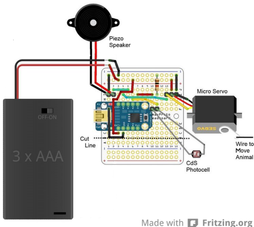
Figure 6-32. The Trinket Toy Animal wiring diagram
