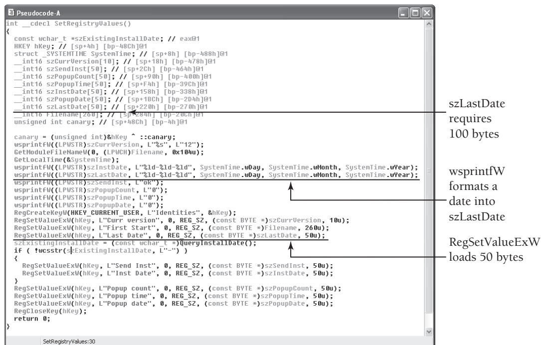
Figure 10-13: Decompile using the Hex-Rays plug-in to create Registry values
