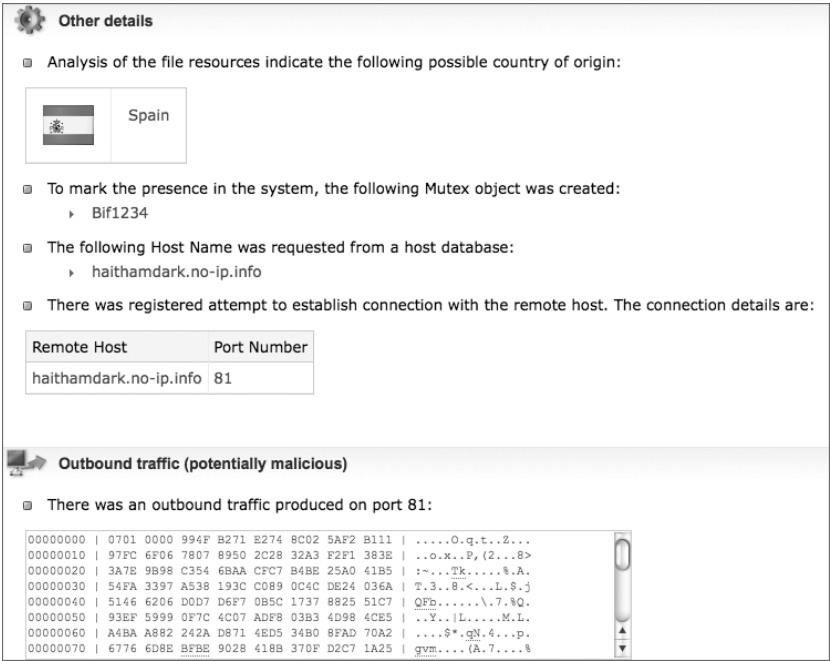
Figure 4-8: ThreatExpert's country of origin and network traffic results
