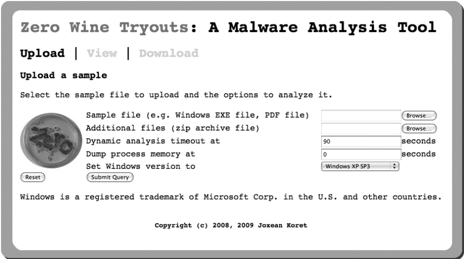
Figure 8-5: The web interface for ZeroWine Tryouts
