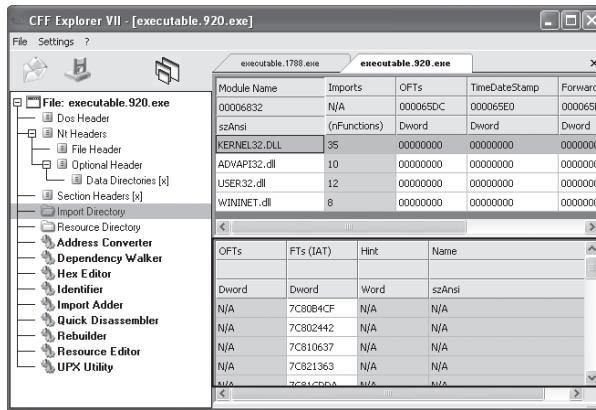
Figure 16-8: The malware's IAT is not rebuilt, perhaps due to packing
