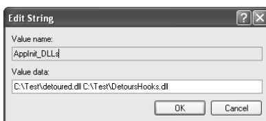
Figure 9-14: Using AppInit_DLLs to load your DLLs
