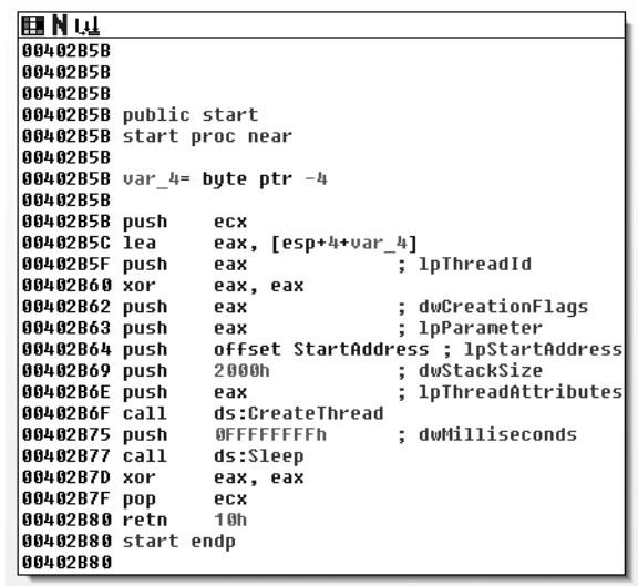
Figure 16-11: The malware in IDA Pro after importing IAT information
