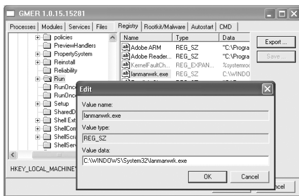
Figure 10-5: Finding and deleting hidden Registry keys
