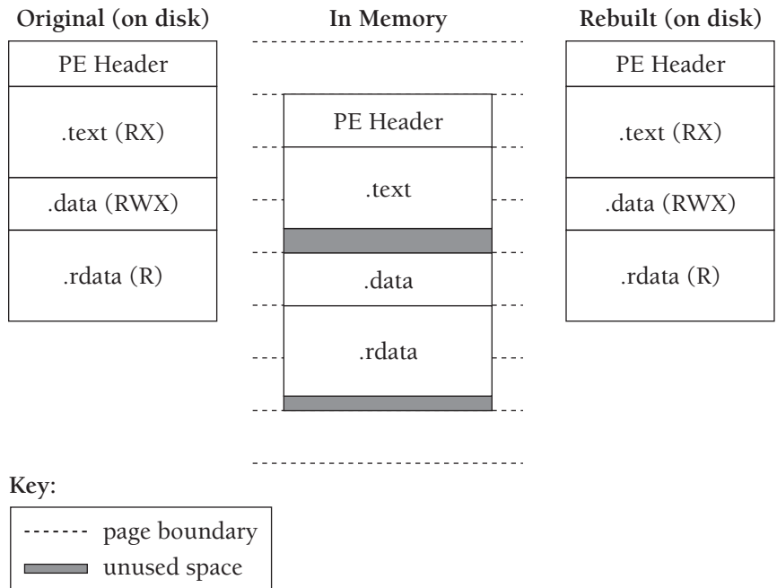
Figure 16-6 Executables expand in memory due to section alignment
