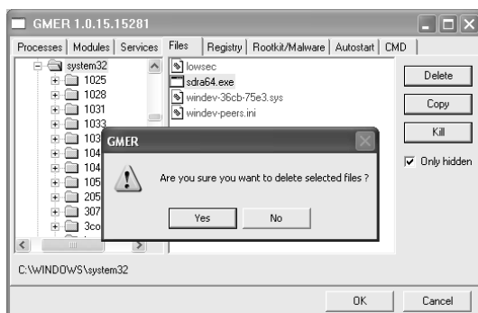
Figure 10-4: Finding and deleting hidden files
