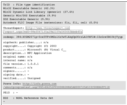
Figure 4-3: VirusTotal's extra information section
