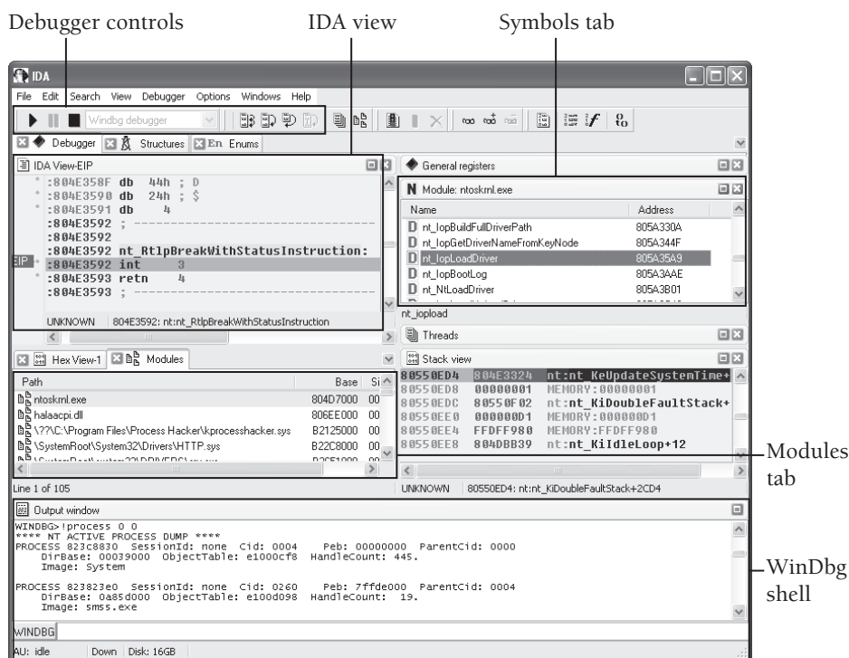
Figure 14-18: Debugging a remote kernel with IDA Pro
