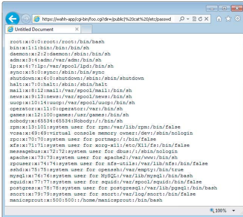
Figure 10-2: A successful command injection attack
