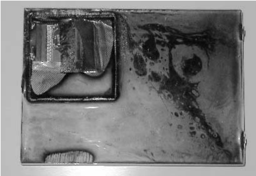
Figure 16.2: The 4758 partially opened showing (from top left downward) the circuitry, aluminium electromagnetic shielding, tamper sensing mesh and potting material (courtesy of Frank Stajano)
