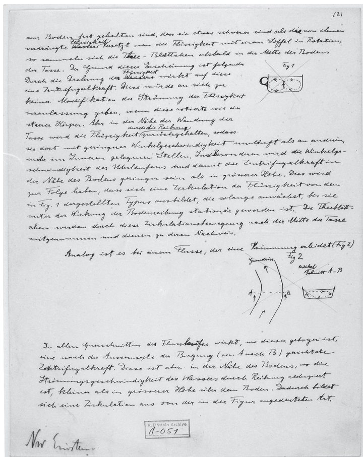
The original second manuscript page of "The Cause and Formation of Meanders."
