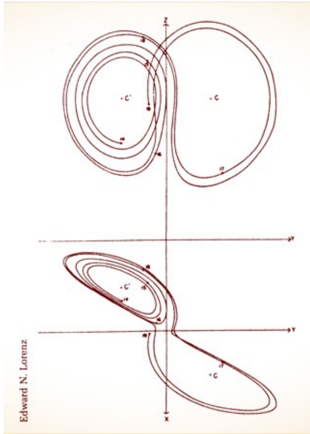
THE FIRST STRANGE ATTRACTOR. In 1963 Edward Lorenz could compute only the first few strands of the attractor for his simple system of equations. But he could see that the interleaving of the two spiral wings must have an extraordinary structure on invisibly small scales.
