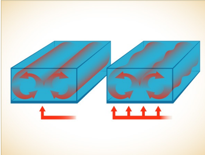
A ROLLING FLUID. When a liquid or gas is heated from below, the fluid tends to organize itself into cylindrical rolls ( left ). Hot fluid rises on one side, loses heat, and descends on the other side—the process of convection. When the heat is turned up further ( right ), an instability sets in, and the rolls develop a wobble that moves back and forth along the length of the cylinders. At even higher temperatures, the flow becomes wild and turbulent.
