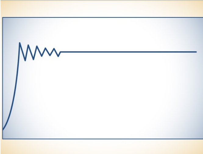
A population reaches equilibrium after rising, overshooting, and falling back.
