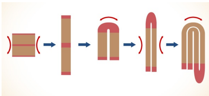
SMALE'S HORSESHOE. This topological transformation provided a basis for understanding the chaotic properties of dynamical systems. The basics are simple: A space is stretched in one direction, squeezed in another, and then folded. When the process is repeated, it produces a kind of structured mixing familiar to anyone who has rolled many-layered pastry dough. A pair of points that end up close together may have begun far apart.
