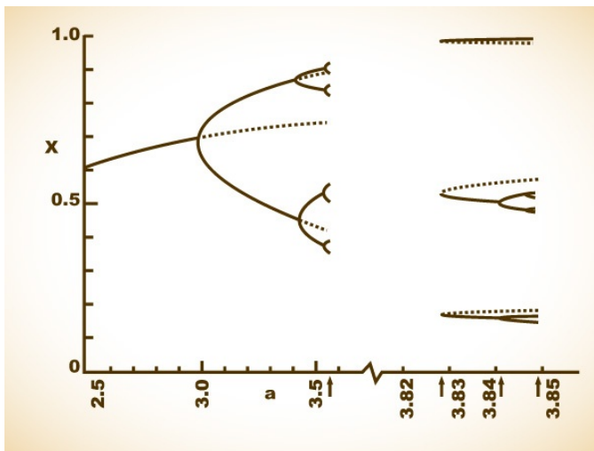
The outline of the bifurcation diagram as May first saw it, before more powerful computation revealed its rich structure.
