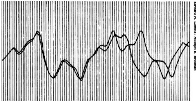
HOW TWO WEATHER PATTERNS DIVERGE. From nearly the same starting point, Edward Lorenz saw his computer weather produce patterns that grew farther and farther apart until all resemblance disappeared. (From Lorenz’s 1961 printouts.)
