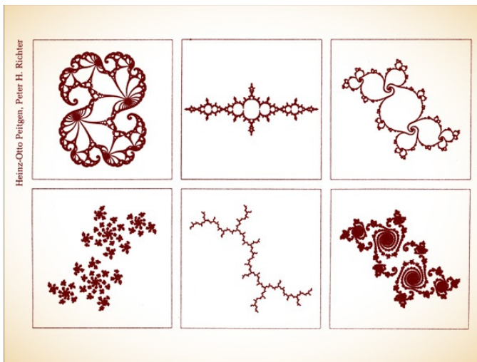
AN ASSORTMENT OF JULIA SETS.
