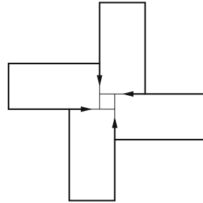
The second winged square derived from the winged shape of area 73 in the margin on page 23. It represents the solution (6, 3, 1) .
