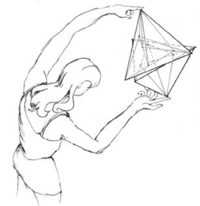
“Touching simplices”
