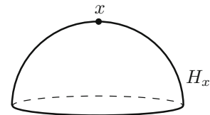
An open hemisphere in S^2
