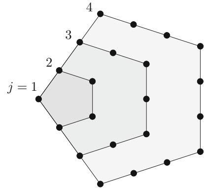
Pentagonal numbers
