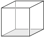
Familiar polytopes: tetrahedron and cube
