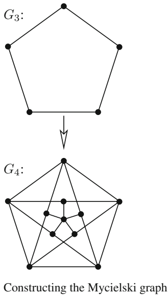
Constructing the Mycielski graph
