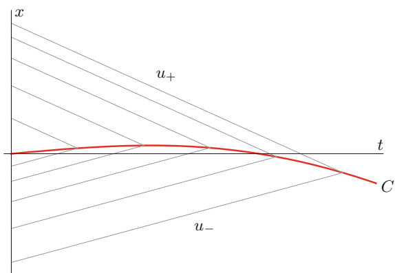
Fig. 10.3 Shock curve with solutions u_{\pm} on either side
