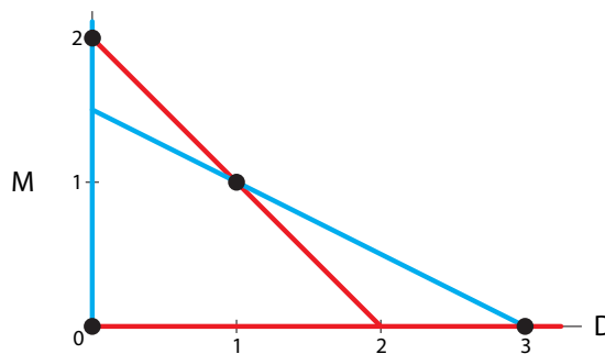
Figure 3.24: Nullclines for the second deer–moose model (equation (3.4)).
