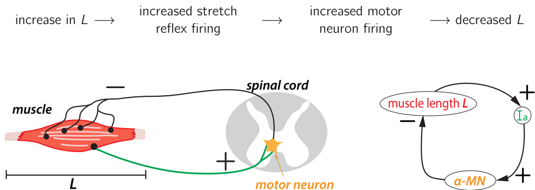
Figure 4.17: Left: There is a simple stretch reflex arc that runs from a muscle to the motor neurons that control it. Right: Schematic of the arc shows that it is a negative feedback loop.
