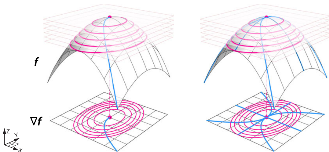
Figure 7.58: When f has a local maximum, trajectories (shown in blue) that follow the gradient vector field \nabla f will climb the hill defined by f(X, Y) as rapidly as possible (the steepest ascent).
