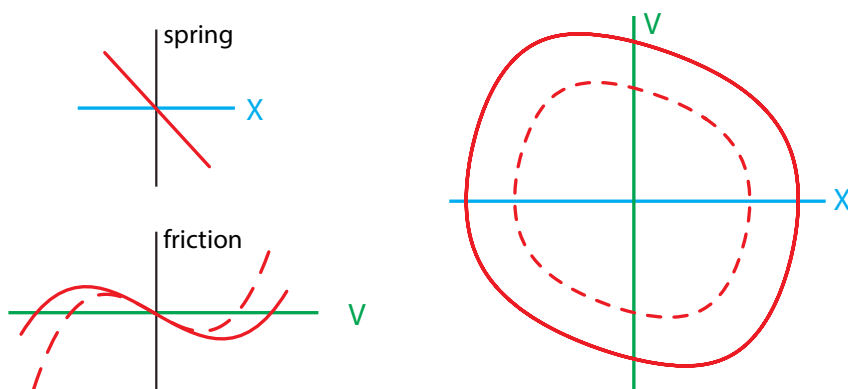
Figure 4.9: Blowing harder. Left: The solid lines show the forces in the Rayleigh clarinet model, under the "blowing harder" condition. The dotted line represents the model without blowing harder. Right: Limit cycle attractors for the two models. Note similarity of shape.
