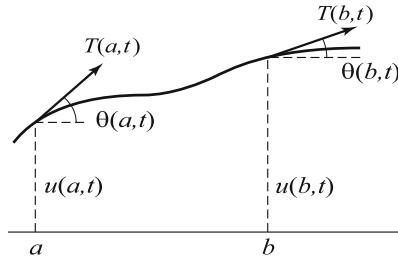
Figure 1.13 Displaced string with tension forces shown
