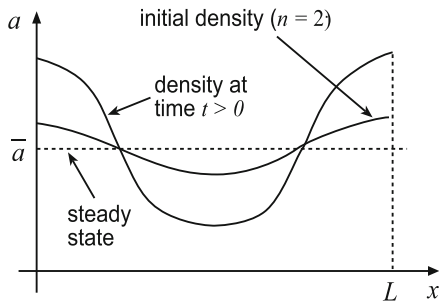
Figure 5.5 Plot showing the growing amoeba density at time t when the uniform state is unstable to local perturbations in the mode n = 2
