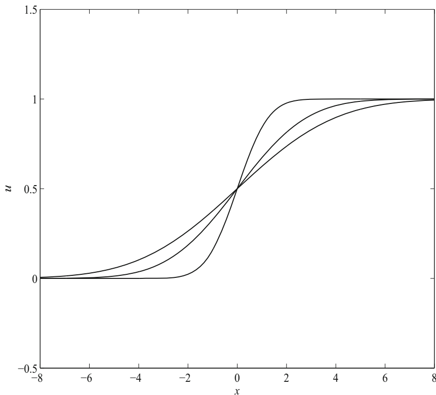
Figure 2.1 Temperature profiles u = \frac{1}{2} \left( 1 + \operatorname{erf} \left( x / \sqrt{4kt} \right) \right) at three different times t when the initial temperature is a step function and k = 1 . As time increases, the profiles are smearing out
