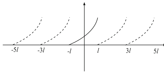
Figure 3.3 A function f defined on (-l, l) ( solid ) and its 2l -periodic extension ( dashed )
