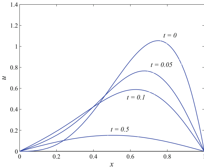
Figure 4.1 Temperature profiles in Example 4.4 at different times. As t \rightarrow \infty the temperature approaches the steady state solution, u \equiv 0
