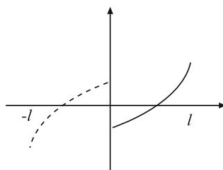
Figure 3.5 A function f defined on (0, l) ( solid ) and its odd extension ( dashed ) to (-l, l)
