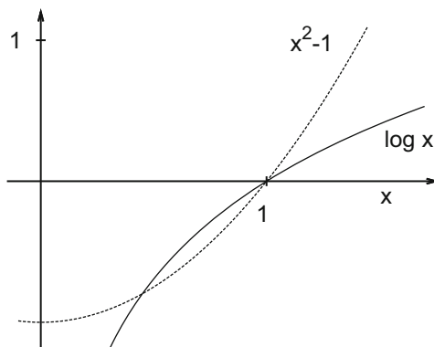
Fig. 4.6 Graphs of the functions in Example 4.9. The ratio of values is equal to the ratio of slopes as x tends to 1
