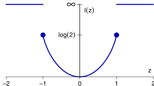
Fig. 23.1 Rate function I(z) from (23.6)
