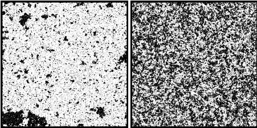
Fig. 18.5 Equilibrium states of the Ising model on an 800 \times 800 grid (black dot = spin +1). Left side : below the critical temperature ( \beta > \beta_c ); Right side : above the critical temperature
