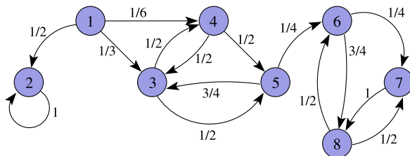
Fig. 17.1 Markov chain with eight states. The numbers are the transition probabilities for the corresponding arrows . State 2 is absorbing, the states 1, 3, 4 and 5 are transient and the states 6, 7 and 8 are (positive) recurrent
