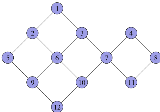
Fig. 19.14 Graph with enumerated nodes
