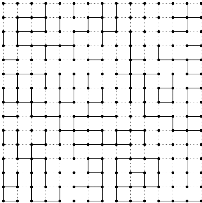
Fig. 2.1 Percolation on a 15 \times 15 grid, p = 0.42
