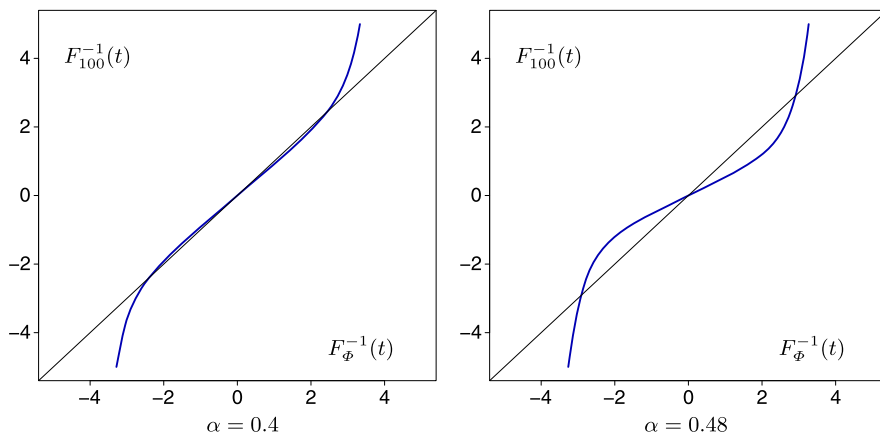
Fig. 15.2 Q-Q-plots for S_{100}^* from Example 15.52 with \alpha = 0.4 (left) and \alpha = 0.48 (right). The abscissa shows the quantiles of the standard normal distribution. For convenience, also the diagonal is drawn
