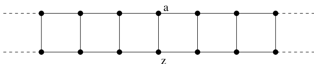
Fig. 19.15 Simple ladder graph
