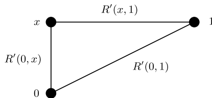
Fig. 19.8 Reduced network with three nodes
