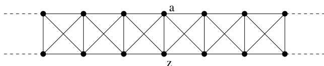
Fig. 19.16 Crossed ladder graph
