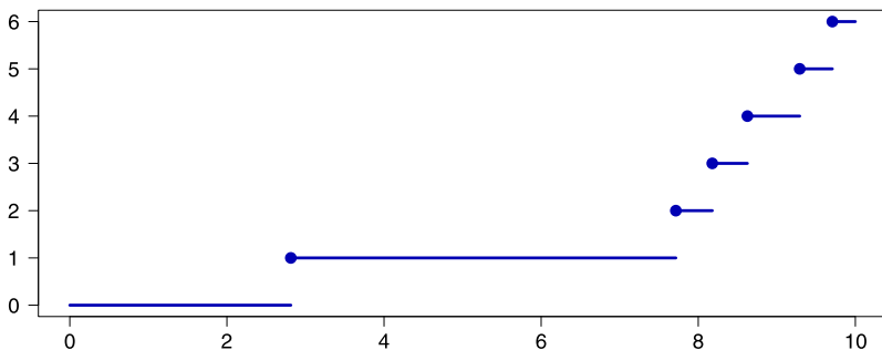
Fig. 5.1 Simulation of a Poisson process with rate \alpha = 0.5
