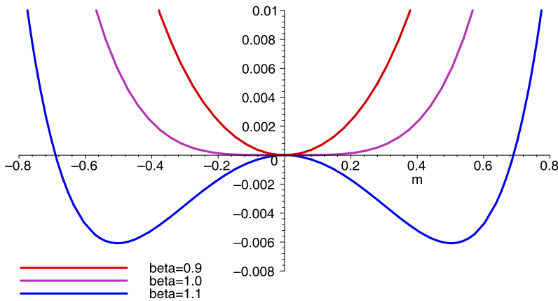
Fig. 23.2 The shifted free energy F^\beta(m) - F^\beta(0) of the Weiss ferromagnet without exterior field ( h = 0 )
