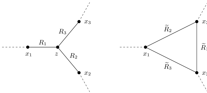
Fig. 19.9 Star–triangle transformation
