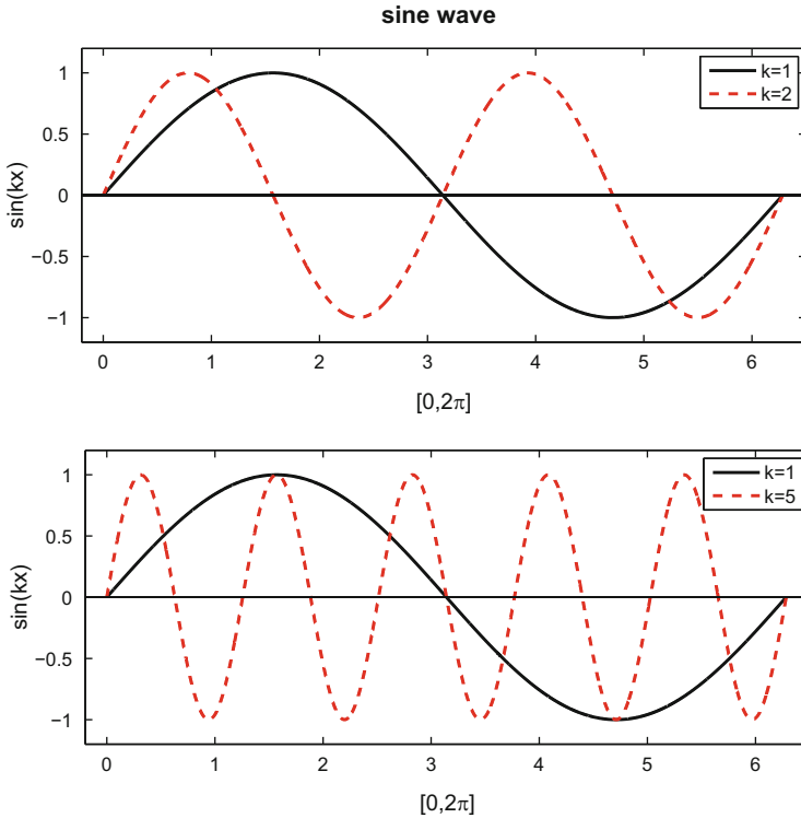
Fig. 10.1 Sine cycles of different frequencies (Example 10.5)
