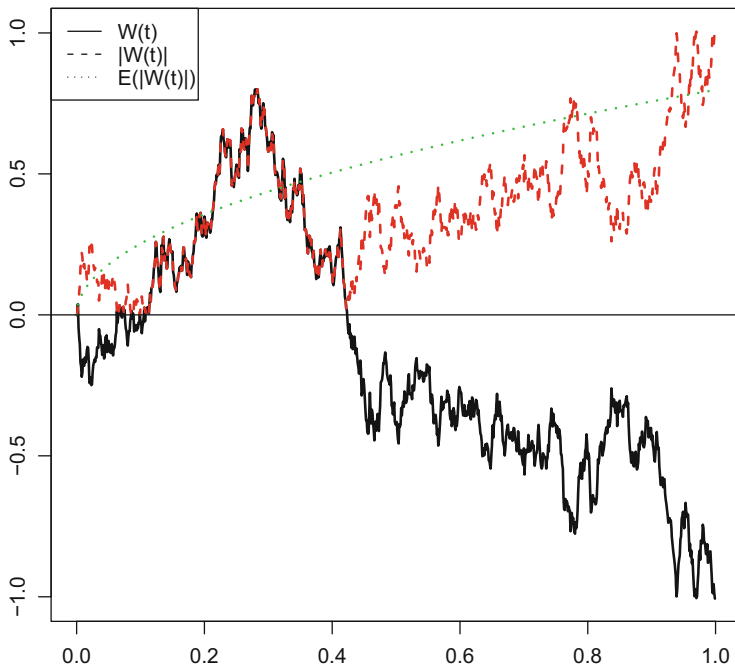
Fig. 7.6 WP and reflected WP along with expectation
