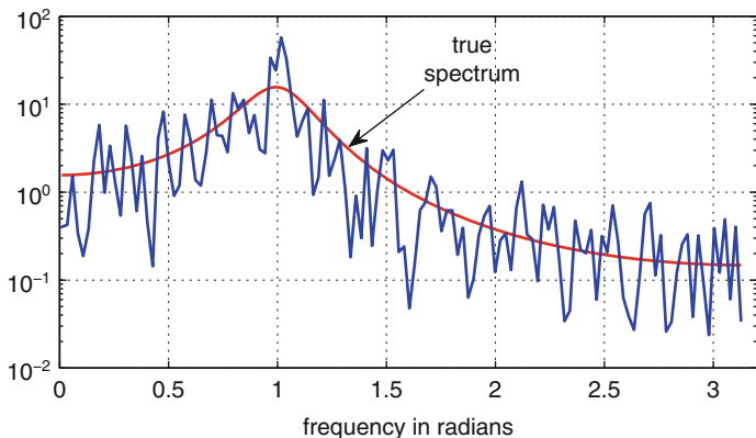
Fig. 6.3 Raw periodogram of an AR(2) process ( X_t = 0.9X_{t-1} - 0.7X_{t-2} + Z_t with Z_t \sim \text{WN}(0, 1) , T = 200 )
