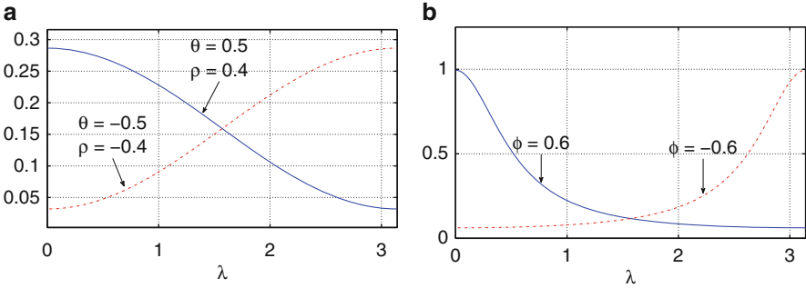
Fig. 6.1 Examples of spectral densities with Z_t \sim \text{WN}(0, 1) . (a) MA(1) process. (b) AR(1) process
