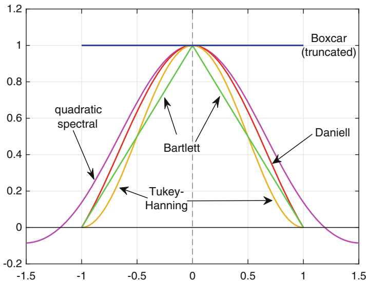
Fig. 4.6 Common kernel functions
