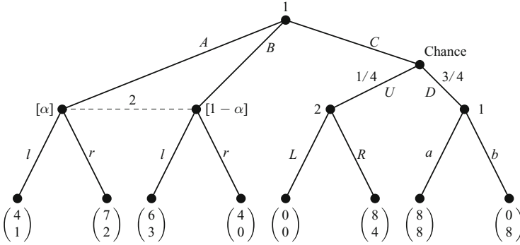
Fig. 4.8 The extensive form game of Fig. 4.1
