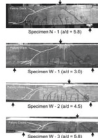
Fig. 13—Photographs of asymmetric tests after failure for all specimens a/d = 1.7 for right side; a/d ratios listed within figure refer to left side).
