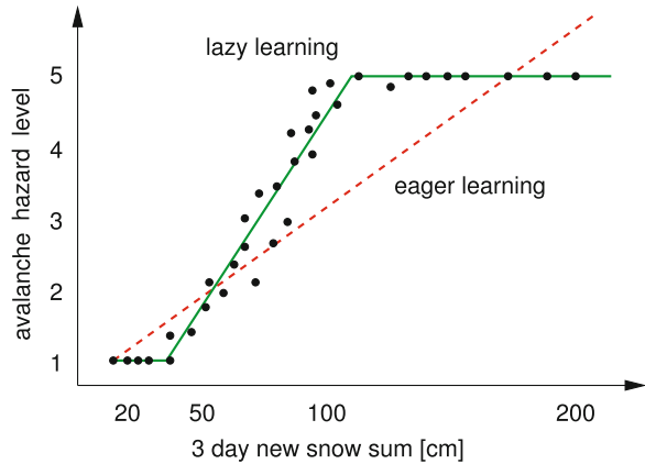
Fig. 8.20 To determine avalanche hazard, a function is approximated from training data. Here for comparison are a local model ( solid line ), and a global model ( dashed line )
