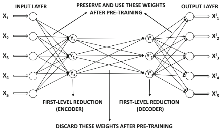
Figure 4.9: This architecture allows the first-level representations in the encoder and decoder to be significantly different. It is helpful to compare this architecture with that in Figure 4.8(a).
